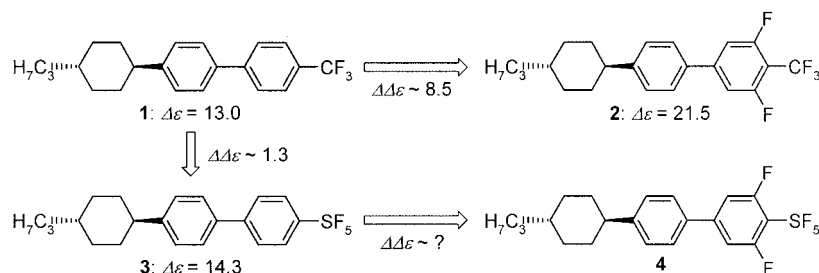
Scheme 1. Increase in the dielectric anisotropies ( \Delta\epsilon ) of liquid crystals induced by the replacement of \text{CF}_3 by the \text{SF}_5 group ( 1 \rightarrow 3 ) and by difluorination of the ortho positions of the polar terminal group ( 1 \rightarrow 2 ).
