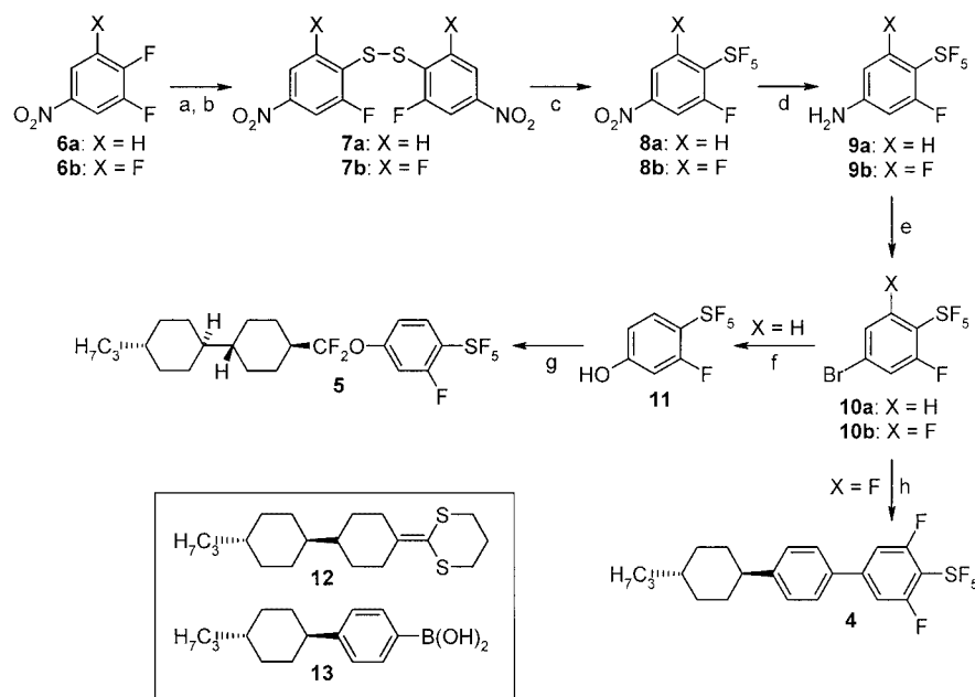
Scheme 2. Synthesis of the liquid crystals 4 and 5 ; reagents and conditions: a) \text{Na}_2\text{S}\cdot 9\text{H}_2\text{O} , DMSO, room temp. \rightarrow 50 °C; b) \text{NaBO}_4\cdot 3\text{H}_2\text{O} , HOAc, room temp. ( 7a : 63%, 7b : 77%); c) 10% \text{F}_2/\text{N}_2 , \text{CH}_3\text{CN} , -3 \rightarrow 0 °C ( 8a : 9%, 8b : 4.6%); d) cat. Raney Ni, \text{H}_2 , THF, room temp., 1 bar ( 9a : 95%, 9b : 95%); e) 1. \text{NaNO}_2 , 47% HBr, 0–5 °C; 2. CuBr, 85 °C ( 10a : 51%, 10b : 49%); f) 1. t\text{BuLi} , \text{Et}_2\text{O} , -70 °C; 2. \text{B}(\text{OMe})_3 ; 3. HOAc, \text{H}_2\text{SO}_4 , 30% \text{H}_2\text{O}_2 , -20 \rightarrow 35 °C (crude product used for next step); g) 1. 12 , \text{CF}_3\text{SO}_3\text{H} , \text{CH}_2\text{Cl}_2 , 0 °C (5 min) \rightarrow room temp. (30 min) \rightarrow -70 °C; 2. 11 , \text{NET}_3 , \text{CH}_2\text{Cl}_2 , -70 °C; 3. \text{NET}_3\cdot 3\text{HF} , -70 °C; 4. \text{Br}_2 , \text{CH}_2\text{Cl}_2 , -70 \rightarrow -10 °C (7%); h) 13 , \text{NaBO}_2\cdot 8\text{H}_2\text{O} , \text{H}_2\text{O} , THF, cat. Pd( \text{PPh}_3 ) 4 , reflux, 18 h (16%).
