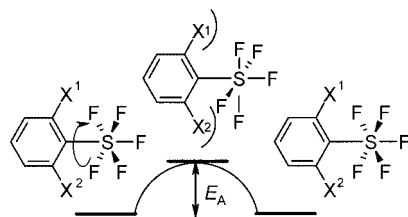
Scheme 3. The activation barriers, E_A , for the rotation of the SF 5 group around the central C-S bond: 18 : 1.8 kcal mol -1 ; 19 : 4.4 kcal mol -1 ; 20 : 7.8 kcal mol -1 . [13]
